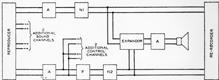
FIG. 6. Block schematic of circuit used for enhancing and re-recording.
